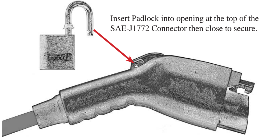
Figure 1. Locking the SAE-J1772 Connector with padlock included.
