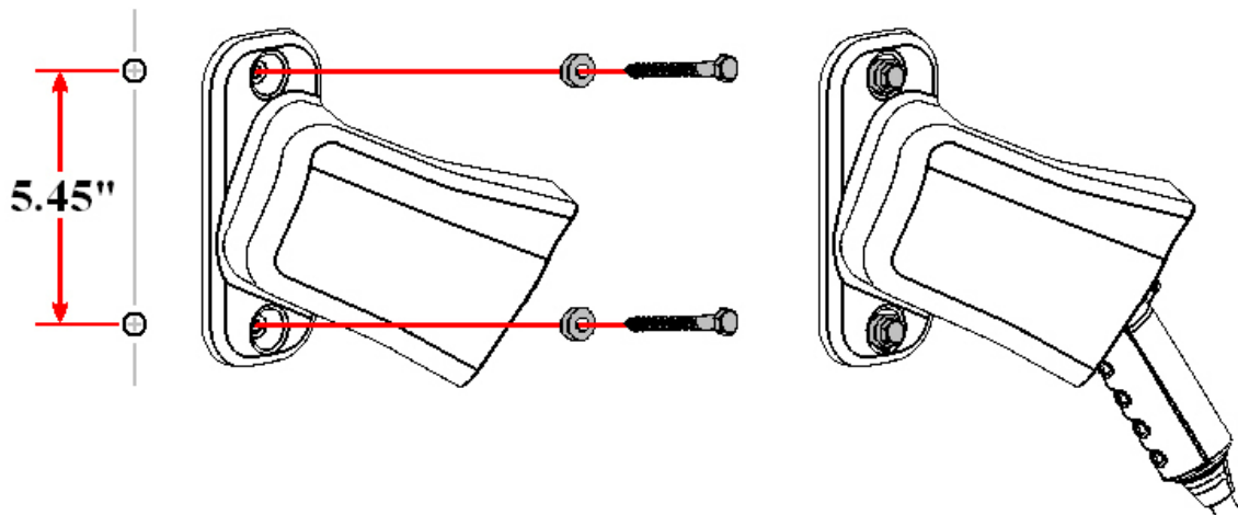
Figure 1. Mounting the Connector Holster using the exterior wood screws and washers
